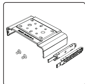
Slide Mount Bracket, Guide Rails and Screws
